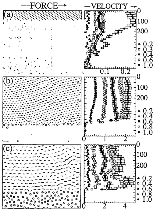
FIG. 1. Forced flow of bubble arrays: Images of size 886 \times 675 \mu\text{m}^2 show flow under force F produced by gradient current I_G = 0.6 A at (a) hexatic glass density \rho = 3935 \text{ mm}^{-2} over time t = 45 sec, (b) hexatic \rho = 1862 \text{ mm}^{-2} over t = 6 sec, (c) liquid \rho = 792 \text{ mm}^{-2} over t = 6 sec. Circles represent Permalloy sites. Each line represents motion of one bubble in the time period. Shown to the right of each image are measured velocity profiles at five values of F indicated by I_G in A: Plots show velocity parallel to F in \mu\text{m}/\text{sec} vs position from top of image in \mu\text{m} .
