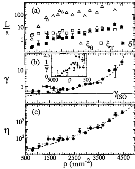
FIG. 4. (a) Measured widths \delta of the shear region, and orientational ( \xi_\theta ) and translational ( \xi_T ) correlation lengths of the bulk, all in units of average lattice spacing a , vs array density \rho . (b) Frictional drag \gamma in Asec/ \mu m. Solid line is \gamma_{iso} measured for isolated bubbles. Dashed-line fit increases as \gamma \propto \rho e^{g\alpha^* \rho_0 / (\rho_0 - \rho)} from \gamma_{iso} . Inset: A linear plot of 1/\gamma vs \rho . The numbers indicate the observed phase of the array: 1=hexatic glass, 2=nonequilibrium hexatic, 3=equilibrium hexatic, and 4=liquid. (c) Shear viscosity \eta in Asec \mu m. Dashed line is a fit \eta \propto e^{(g\alpha^* + C_1)\rho_0 / (\rho_0 - \rho)} (see text).
