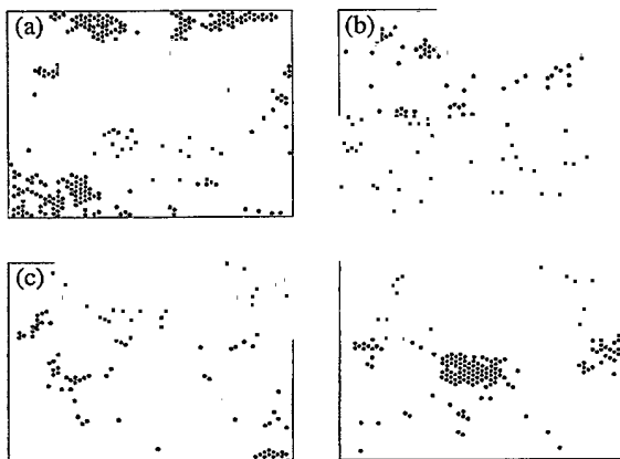
FIG. 3. Sequence of moving bubble images ( 1027\times 768 \mu\text{m}^2 ) for H_{ac}=10.1 Oe and F=1.24\times 10^{-7} dyn. The cutoff velocity is 0.0075 \mu\text{m}/\text{sec} . Each image is averaged over 6 min.
