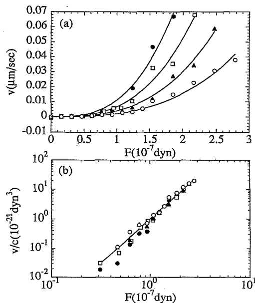
FIG. 1. (a) Velocity-force response of the magnetic bubble array for ac magnetic-field values H_{ac} = 10.1 Oe (open circles), 13.6 Oe (black triangles), 17.2 Oe (open squares), and 20.7 Oe (black circles). The solid lines are power-law fits with v = cF^3 ; c is the fitting parameter. (b) Log-log plot of v/c vs F ; the solid line is v/c = F^3 .
