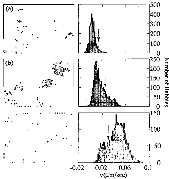
FIG. 2. Distributions of moving bubble clusters and histograms of bubble velocity for H_{ac}=10.1 Oe and (a) F=0.93\times 10^{-7} dyn, (b) F=1.86\times 10^{-7} dyn, and (c) F=2.79\times 10^{-7} dyn. The black dots represent bubbles with velocities above the cutoffs indicated by the arrows on the corresponding histograms. Image sizes are all 1027\times 768 \mu\text{m}^2 .
