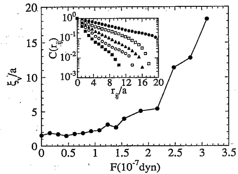
FIG. 4. Velocity-velocity correlation length \xi_v vs force F at H_{ac}=10.1 Oe. The inset shows the velocity-velocity correlation function vs bubble separation at forces 2.79\times 10^{-7} dyn (black dots), 1.86\times 10^{-7} dyn (open squares), 1.24\times 10^{-7} dyn (black triangles), 0.93\times 10^{-7} dyn (open circles), and 0.46\times 10^{-7} dyn (black squares).
