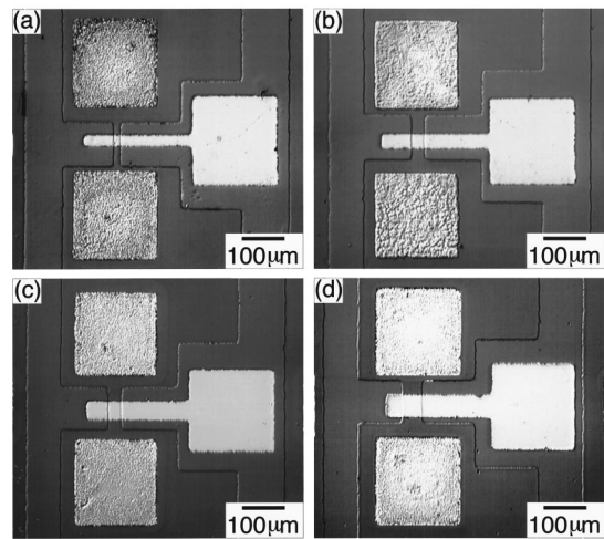
FIG. 3. Micrographs of FETs with various gate lengths L and gate widths Z fabricated by soft lithography. (a) L=26 \mu\text{m} and Z=16 \mu\text{m} ; (b) L=34 \mu\text{m} and Z=30 \mu\text{m} ; (c) L=44 \mu\text{m} and Z=32 \mu\text{m} ; (d) L=52 \mu\text{m} and Z=47 \mu\text{m} .
