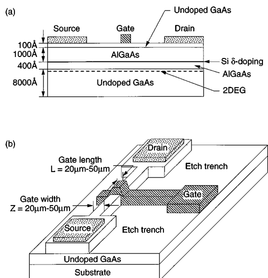
FIG. 1. (a) Schematic cross sectional view of the field effect transistor (FET) to show the growth profile of the GaAs/AlGaAs material. (b) Schematic diagram of GaAs/AlGaAs heterostructure FET.
