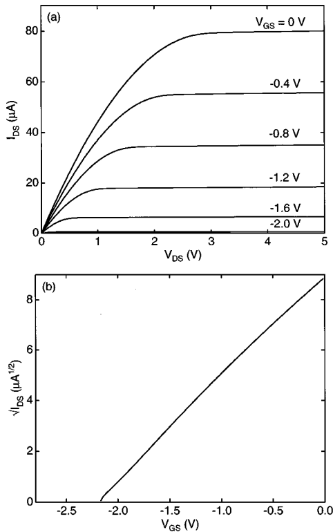
FIG. 4. Performance of a representative FET fabricated by soft lithography. The FET has L = 30 \mu\text{m} and Z = 21 \mu\text{m} . (a) Drain-source characteristics. (b) Transfer characteristics measured at V_{DS} = 4 \text{ V} .
